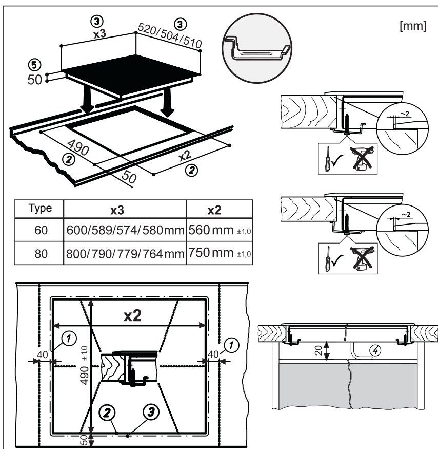
Bracket
