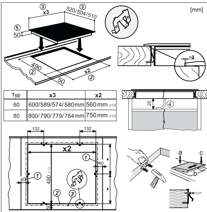
Clips
