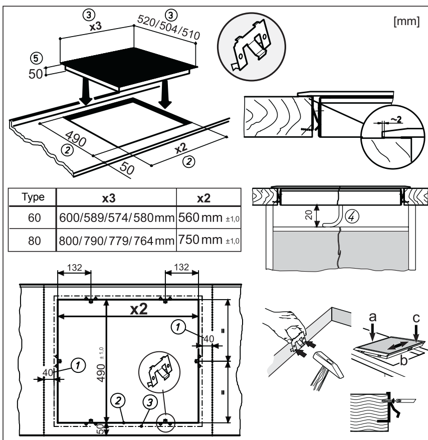
Clips
